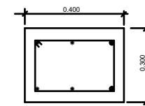
GRADE BEAM DETAILS 6R12 R8@150mm
